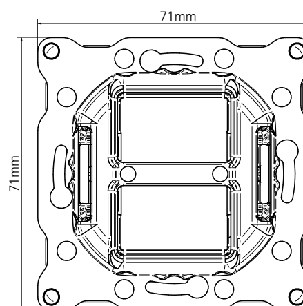
Figure 3. Dimensions, fixation de montage LOCUS.
