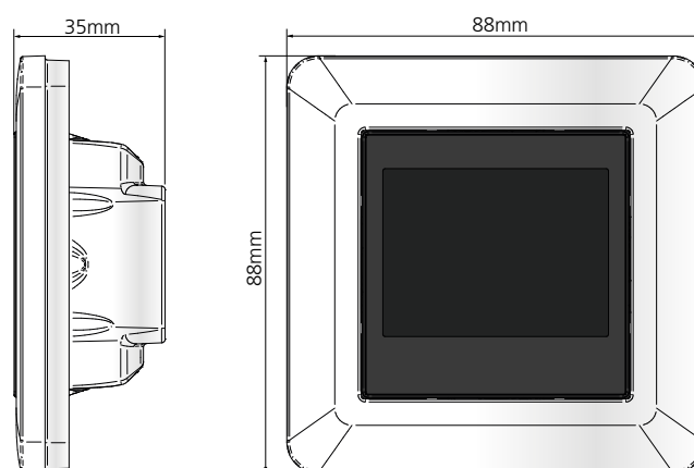
Figure 2. Dimensions, LOCUS.
